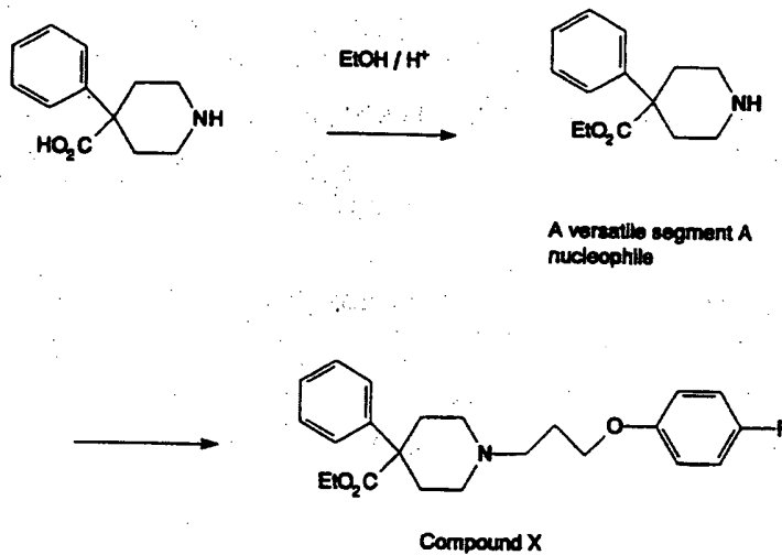
Scheme 14
